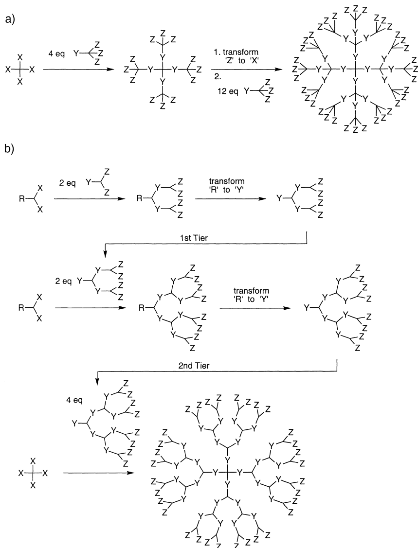
Fig. 1.9 Syntheses of dendrimers: (a) Divergent method, (b) convergent method.
