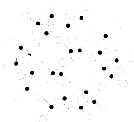
Fig. 1.5 Zeolite structure. The arrangement of \text{AlO}_4 and \text{SiO}_4 tetrahedra which gives the cubo-octahedral cavity in some zeolites and feldspaths. • represents Si or Al. (Reproduced from Advanced Inorganic Chemistry , 3rd edition. F.A. Cotton and G. Wilkinson, Interscience/Wiley, 1972, p. 324.)
