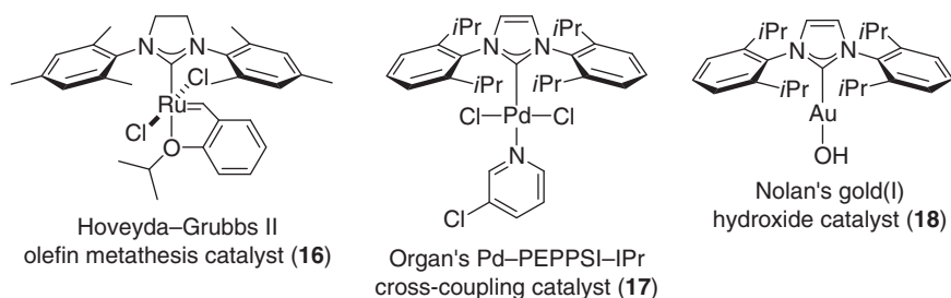
Figure 1.5 Selected examples of important NHC-containing transition metal catalysts.
