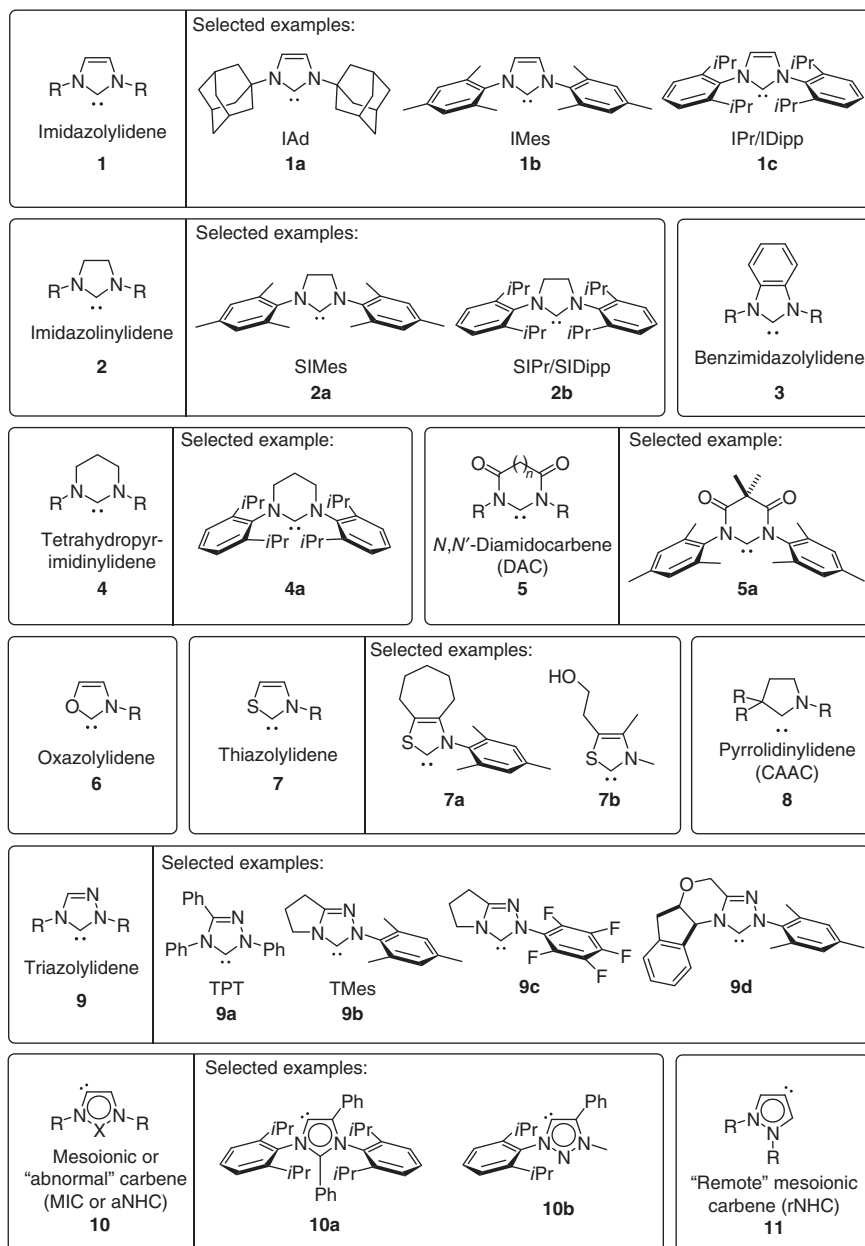
Figure 1.1 Some important classes of NHC with selected examples.
