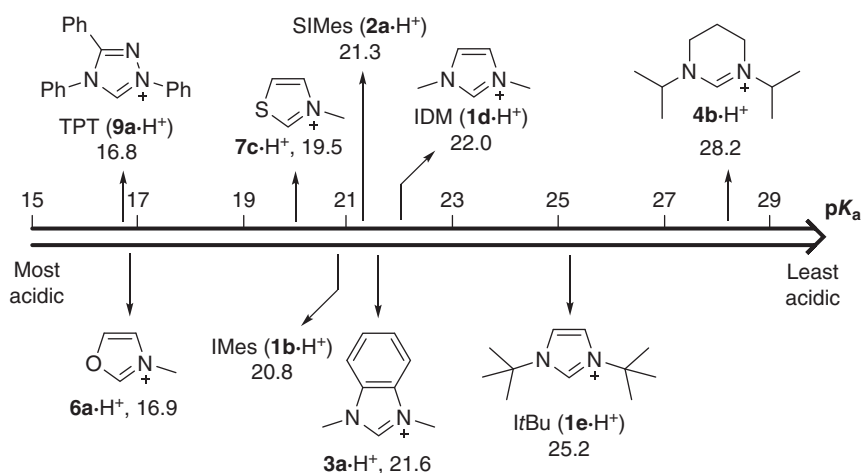
Figure 1.14 Scale showing pK_a values measured in D_2O for representative examples of different classes of NHC.
