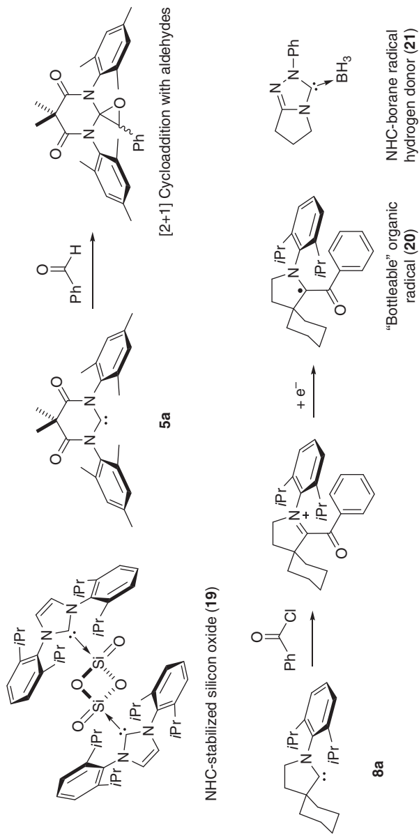
Figure 1.6 Selected examples of adducts between NHCs and non- or semimetallic species.
