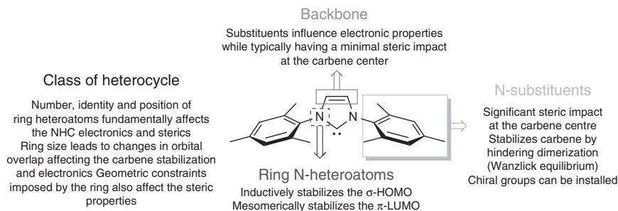
Figure 1.3 General structural features of NHCs exemplified for IMes (1b).
