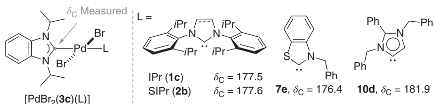
Figure 1.20 ^{13}\text{C} NMR shifts of the carbene carbon of benzimidazolylidene 3c in palladium(II) complexes [\text{PdBr}_2(\mathbf{3c})(\text{L})] measured by Huynh and coworkers.
