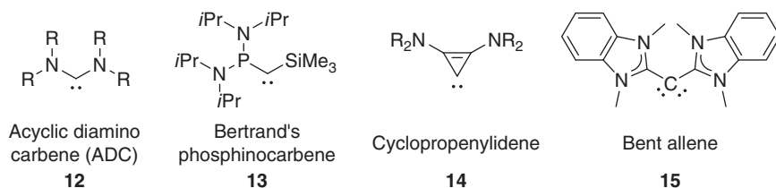
Figure 1.2 Selected related classes of stable carbene.
