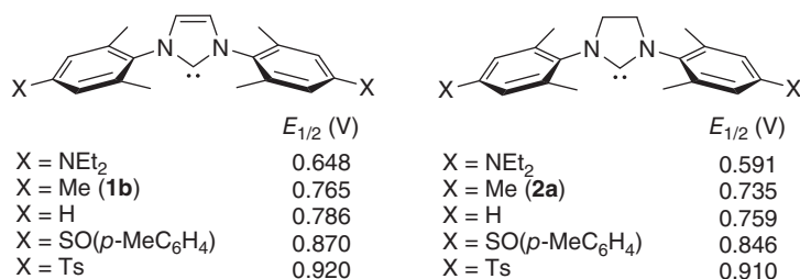
Figure 1.23 Electrochemical measurements on iridium complexes of the form [IrCl(COD)(L)] with different imidazolylidene and imidazolylidene NHCs (measured in 0.1 M NBu 4 PF 6 , referenced to FcMe 8 , scan rate: 100 mV s -1 ).
