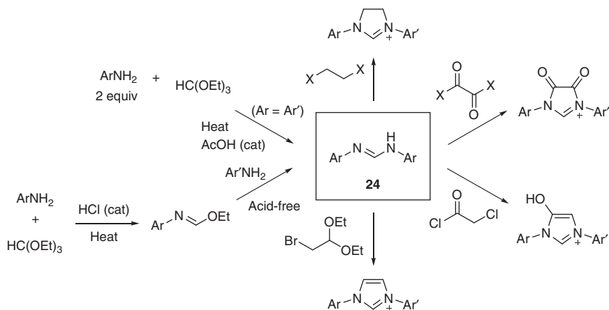
Figure 1.11 Selected synthetic routes to imidazolium salt NHC precursors from formamidines 24 .
