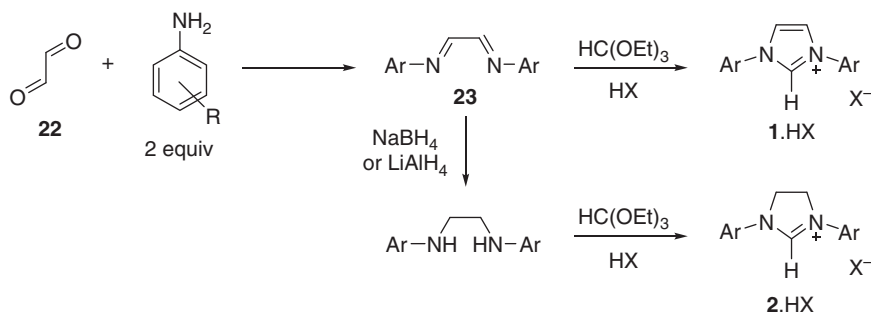
Figure 1.10 Synthesis of imidazolium and imidazolinium salt precursors from glyoxal ( 22 ).
