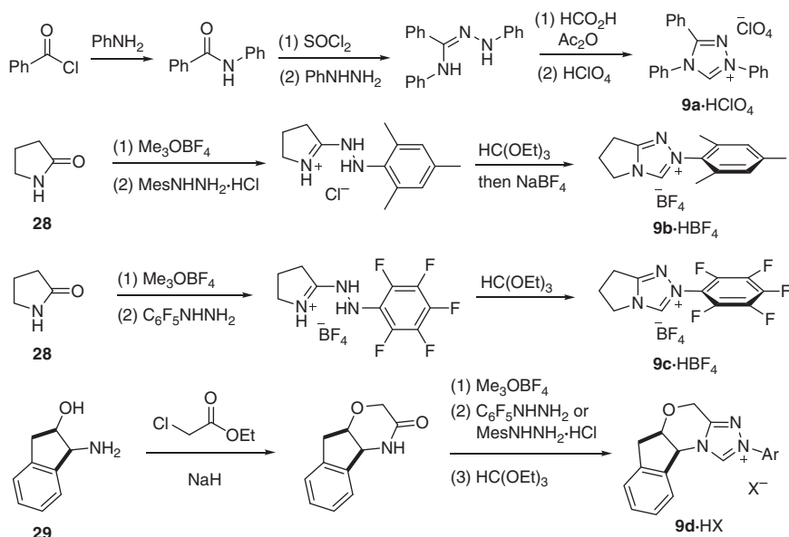
Figure 1.13 Selected synthetic routes to triazolium salt NHC precursors.
