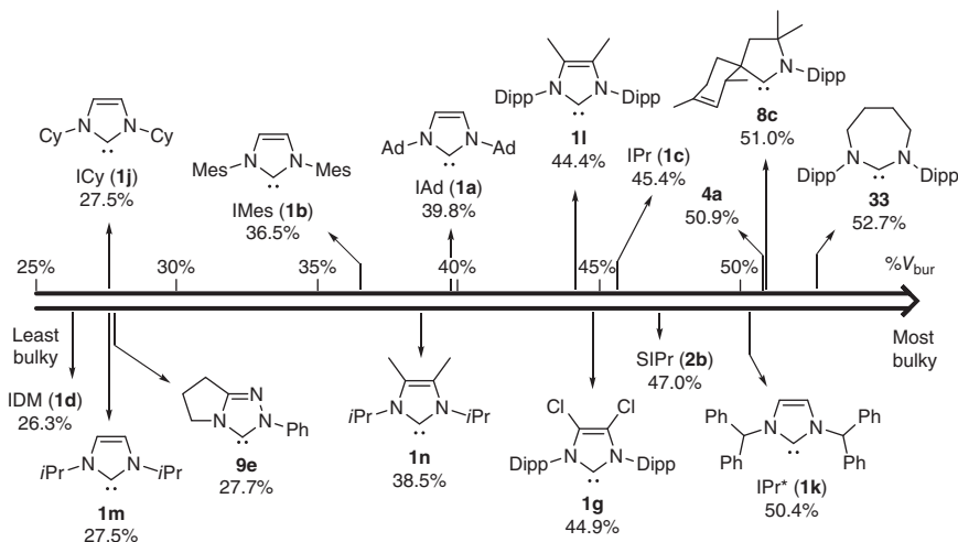
Figure 1.26 Scale showing the variation in % V_{\text{bur}} values for imidazolyliidenes with different nitrogen and backbone substituents.
