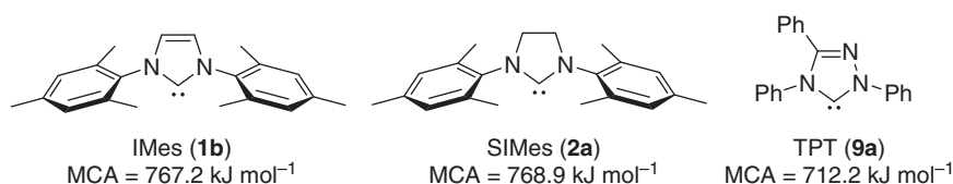
Figure 1.22 Calculations of the MCA of IMes ( 1b ), SIMes ( 2a ), and TPT ( 9a ) by Mayr and coworkers.
