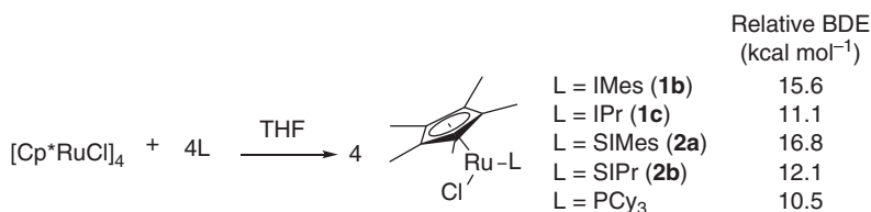
Figure 1.7 Comparison of the binding strength of different NHCs and PCy 3 in [Cp*Ru(L)Cl] complexes (L = ligand) by Nolan and coworkers. Source: Hillier et al. 2003 [47]. Reproduced with permission of ACS.
