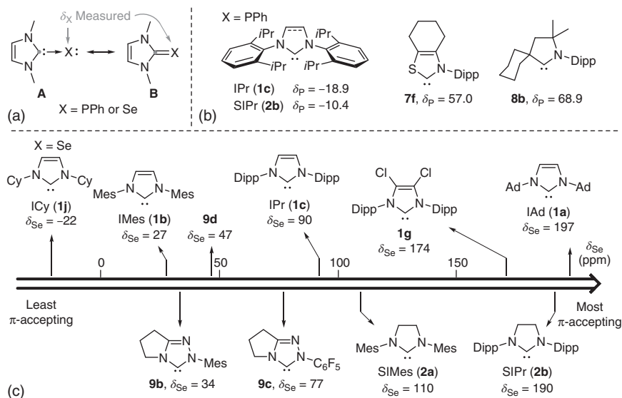
Figure 1.21 (a) Extreme resonance forms A and B of NHC-phosphorus and NHC-selenium adducts. (b) ^{31}\text{P} NMR shifts of NHC-phosphorus adducts for selected NHCs (measured in \text{C}_6\text{D}_6 ). (c) Scale showing ^{77}\text{Se} NMR shifts for selected NHC-selenium adducts (measured in \text{CDCl}_3 ).
