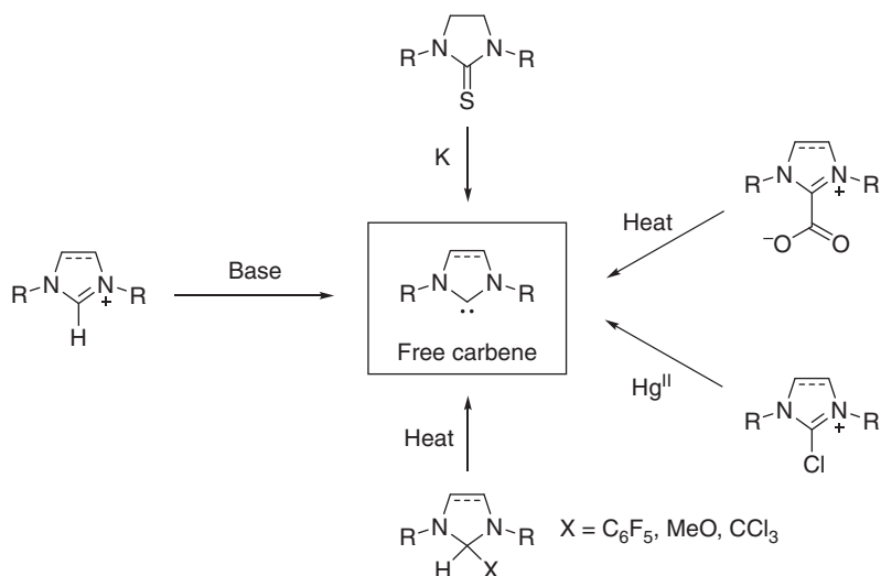
Figure 1.9 Some commonly employed methods of generating free NHCs.
