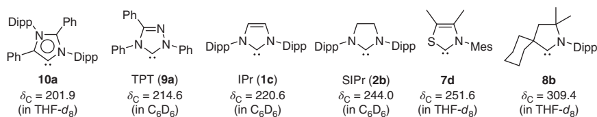
Figure 1.19 ^{13}\text{C} NMR shifts of the carbene carbon in selected free NHCs.
