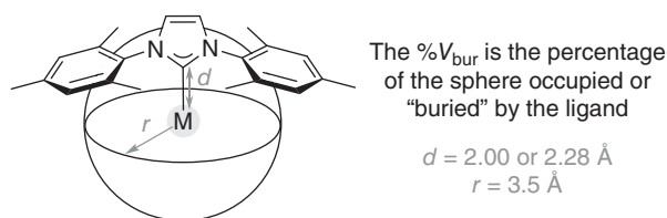
Figure 1.25 Model used to determine the percentage-buried volume (% V_{\text{bur}} ) of NHCs.
