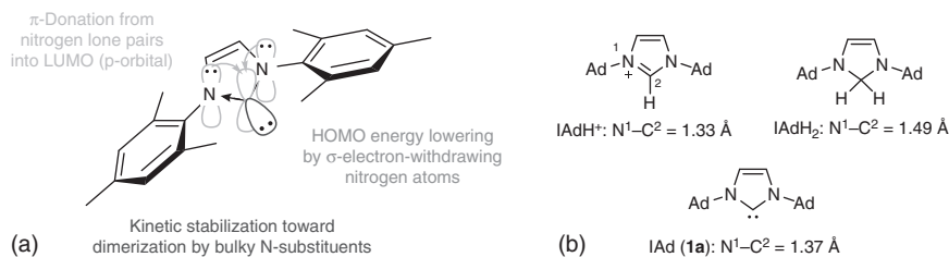
Figure 1.4 (a) Stabilization of the carbene by adjacent ring nitrogens. (b) Comparison of the N^1-C^2 bond lengths in IAd derivatives.
