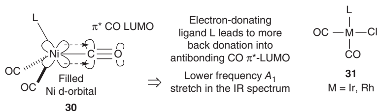
Figure 1.16 The measurement of TEP values.
