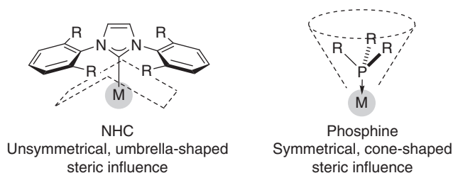
Figure 1.8 Comparing the steric properties of NHCs and phosphines.
