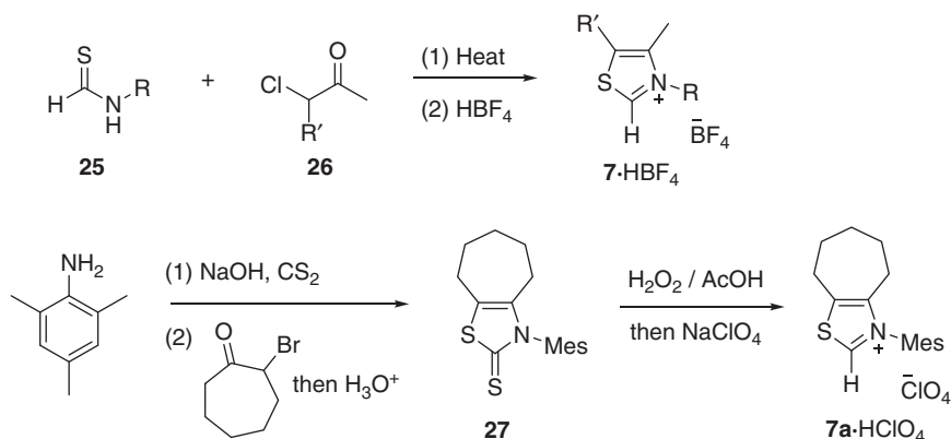
Figure 1.12 Selected synthetic routes to thiazolium salt NHC precursors.
