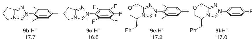
Figure 1.15 Literature pK_a values for azolium salts of some triazolylidene organocatalysts with different N -aryl groups (measured by NMR in D_2O ).
