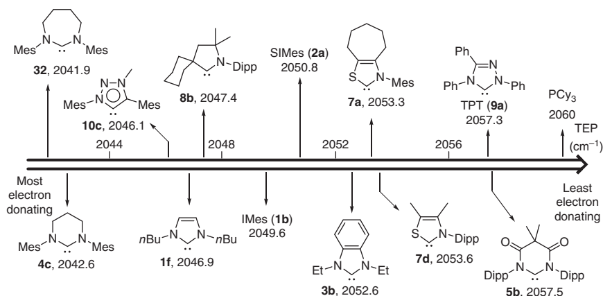
Figure 1.17 Scale showing the range of TEP values measured with different NHCs.
