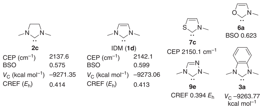
Figure 1.24 Electronic parameters of model NHCs calculated using DFT.
