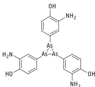
Arsphenamin (trimere Form)
