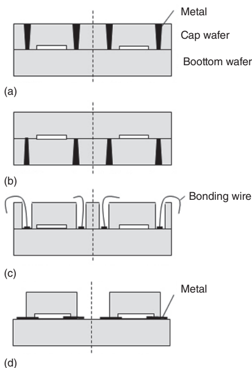
Figure 1.7 Interconnection methods from the packaged MEMS (a) Through-substrate-vias (cap), (b) Through-substrate-vias (bottom), (c) Wire-bonded through-Si vias, (d) Lateral feedthrough.
