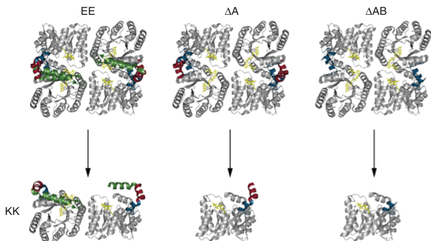
Figure 1.8 Oligomeric state of TtProDH and its site-directed mutants. EE: F10E/L12E variant. ΔA: TtProDH without the N-terminal helix αA. ΔAB: TtProDH without the N-terminal helices αA and αB. KK: D205K/E207K variants of EE, ΔA and ΔAB. The flavin cofactor is shown in yellow, helix αA in green, helix αB in red, and helix αC in blue. Source: Modified from Huijbers et al. [51].
