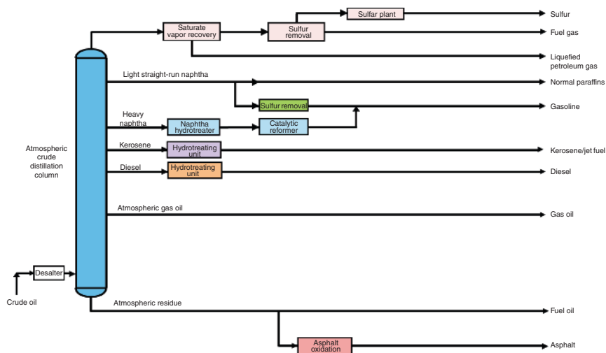
Figure 1.1 Topping and hydroskimming refinery.
