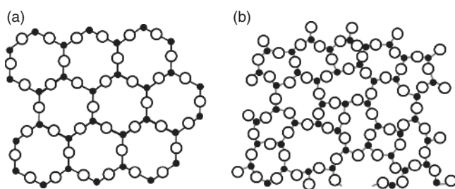
Figure 1.2 Structural motifs in silicon dioxide ( \text{SiO}_2 ): (a) – ordered atomic arrangement in crystalline quartz; (b) – disordered arrangement in amorphous silica. Large open circles and black filled circles indicate oxygen and silicon atoms, respectively.
