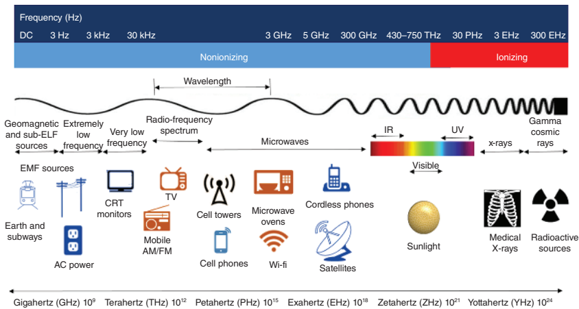
Figure 1.1 Frequency and wavelength ranges in the electromagnetic spectrum, and devices that emit radiation at certain frequencies. Source: Chong Min Koo.
