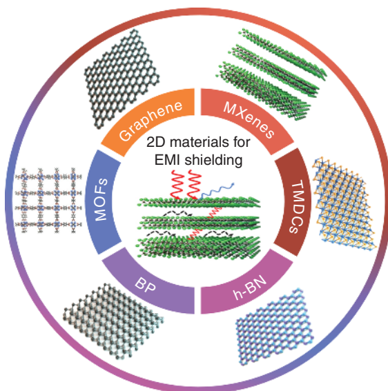
Figure 1.5 Atomic structures of 2D materials used for EMI shielding. The development of these novel 2D materials has provided a breakthrough in replacing conventional conductive metals, which suffer from high density and corrosion susceptibility. Source: Chong Min Koo.
