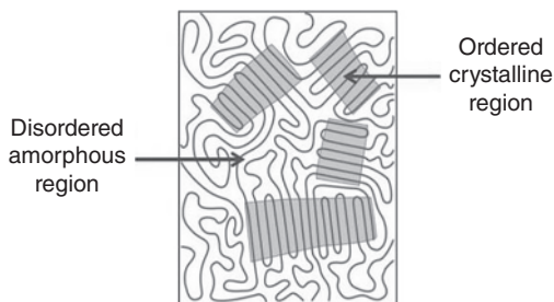
Figure 1.8 Polymeric monocrystals.
