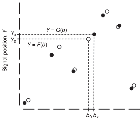
Figure 1.8 Analytical calibration in qualitative analysis: analyte b_0 in a sample (empty points) is identified as analyte b_x in a standard (full points) on the basis of mutual signal positions, Y_0 and Y_x .
