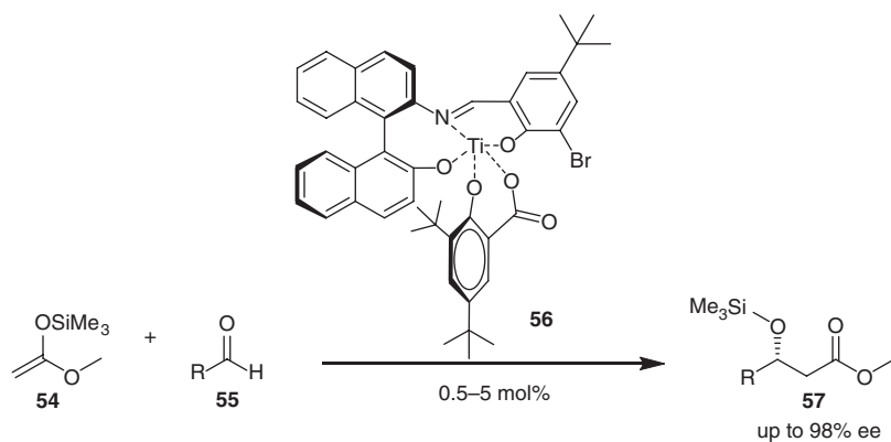
Figure 1.18 Enantioselective aldol reaction with silyl ketene acetals.
