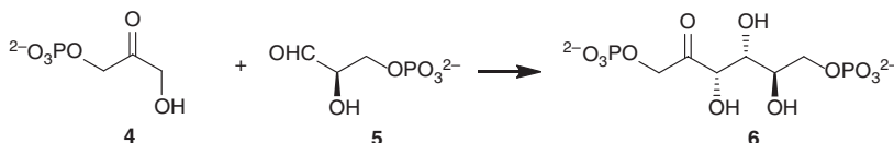
Figure 1.2 Aldolase reaction.
