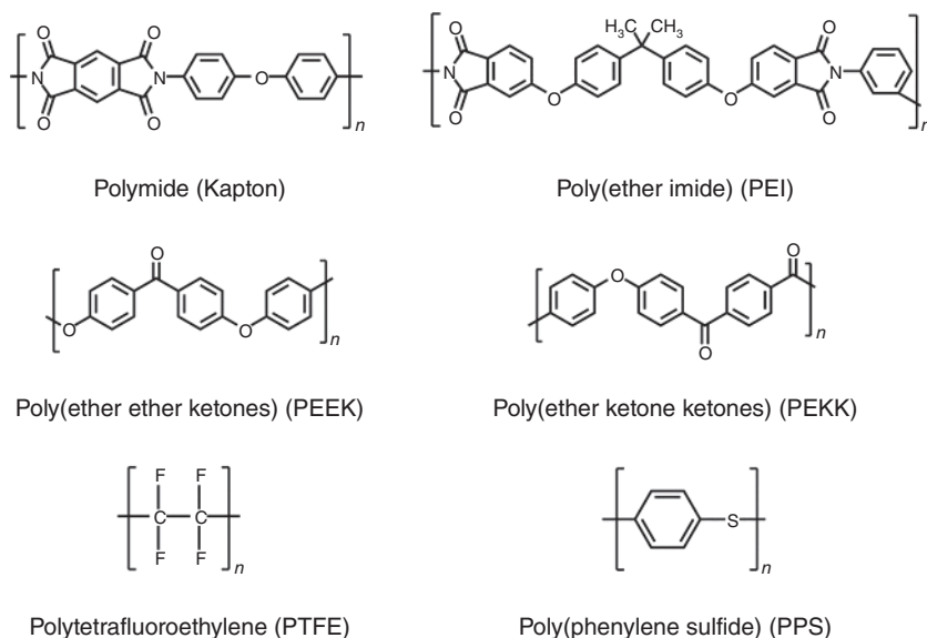
Figure 1.7 The structural formula for several common high-temperature polymers.
