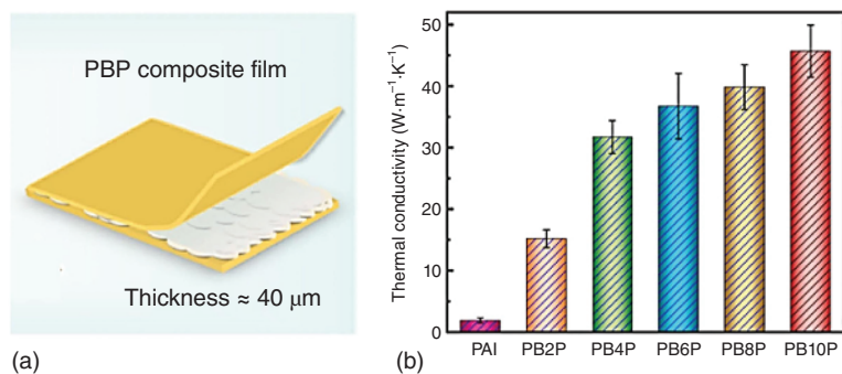
Figure 1.5 (a) Schematic diagram of the structure of PBP composite film. (b) \lambda_{//} of pure PAI and PBP composite films with different numbers of filler layers [33]. Source: Zhou et al. [33]. Reproduced with permission of Elsevier.
