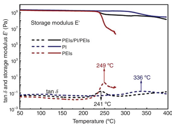
Figure 1.2 E' and \tan \delta as a function of temperature for PI, PEIs, and three-layer PEIs/PI/PEIs films [30]. Source: Niu et al. [30]. Reproduced with permission of Elsevier.
