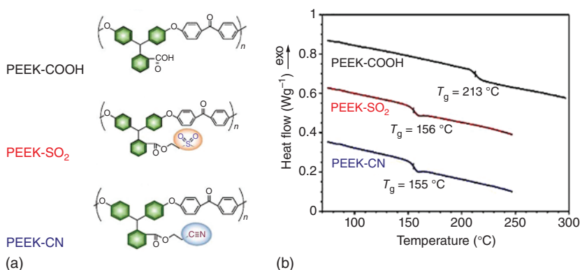
Figure 1.1 (a) Structure formula and (b) DSC of PEEK polymers [29]. Source: Huang et al. [29]. Reproduced with permission of Wiley-VCH.
