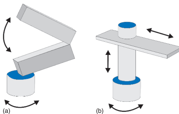
Figure 1.4 Anthropomorphic (a) and cylindrical (b) geometry of robot arms.
