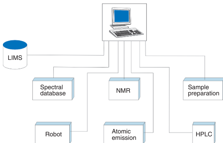
Figure 1.3 Local area network (LAN) to connect analytical instruments, a robot, and a laboratory information management system (LIMS).
