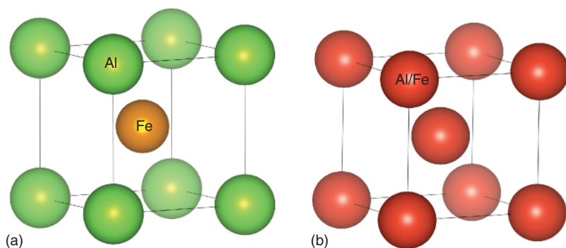
Figure 1.7 The crystal structures of FeAl alloy at (a) low and (b) high temperatures.
