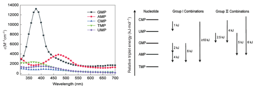
Figure 1.4 Triplet-triplet (T-T) absorption spectra of DNA/RNA nucleotides and scheme of their triplet state energy level.
