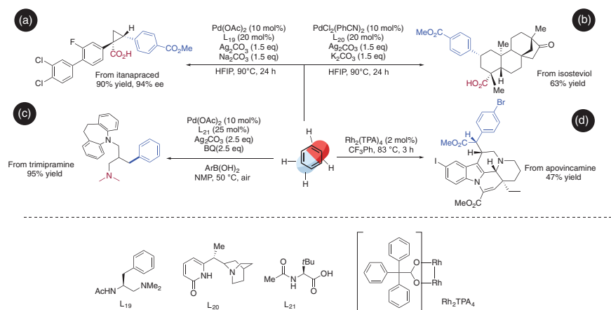
Figure 1.11 Late-stage diversification of aliphatic substrates via C–C bond formation. a) Pd-catalyzed C( sp^3 )-H late-stage arylation of itanaprazed developed by Yu et al. [84] b) Pd-catalyzed C( sp^3 )-H late-stage arylation of isosteviol developed by Yu et al. [85] c) Pd-catalyzed C( sp^3 )-H late-stage arylation of trimipramine developed by Gaunt et al. [86] d) Pd-catalyzed C( sp^3 )-H late-stage alkylation of apovincamine developed by Davies, Beckwith et al. [88].
