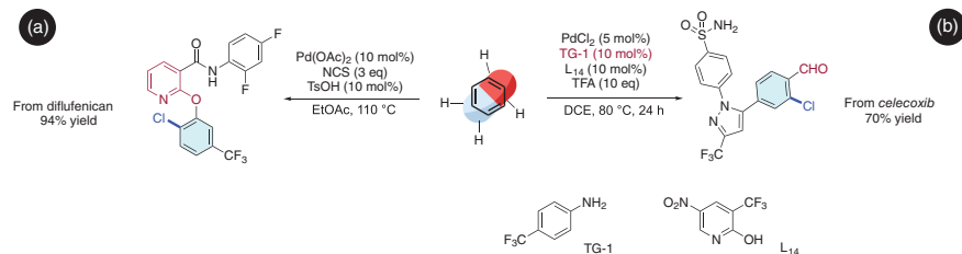
Figure 1.9 Late-stage direct chlorination. a) Pd-catalyzed late-stage chlorination of diflufenican developed by Wu, Wu et al. [67] b) Pd-catalyzed late-stage chlorination of celecoxib developed by Zhang et al. [68].
